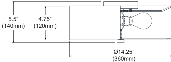
Option A Flush
