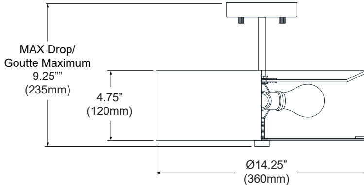
Option B Semi-Flush
